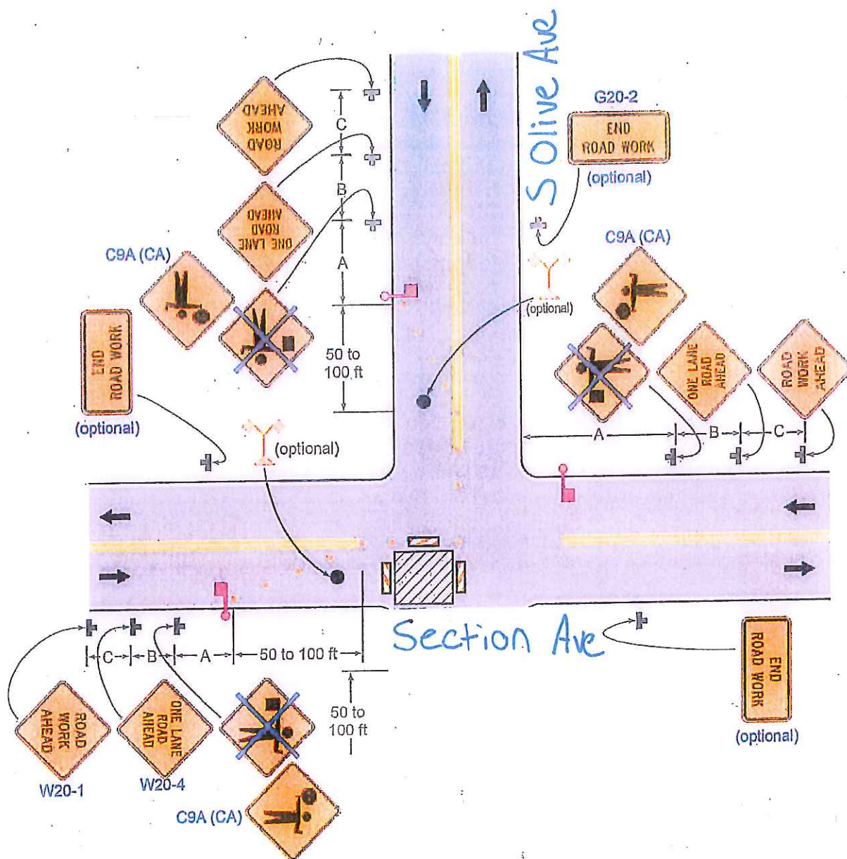
Figure 6H-27. Closure at the Side of an Intersection (TA-27)
